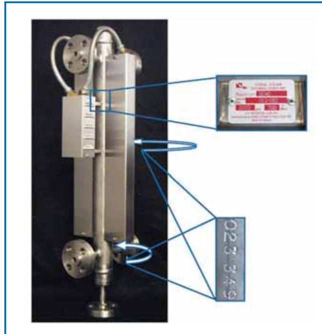
TYPICAL AQUARIAN WATER COLUMN
